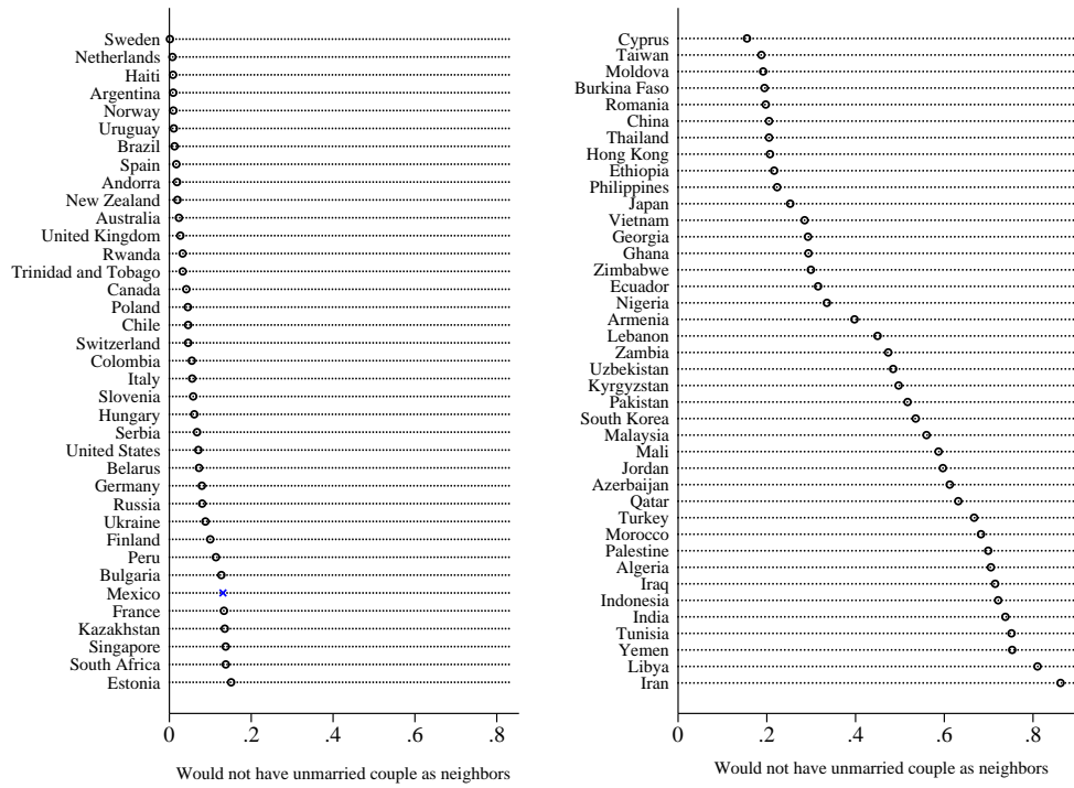
FIGURE 4 Cross-Country Comparison of the Norms around Informal Unions. Notes: The data from this figure comes from the 5 th and 6 th waves of the World Value Survey. For countries that participated in both waves, we use the most recent data. This graph displays the share of respondents ages 40 and above in each country that answered that they would not like to live next to an unmarried couple.
